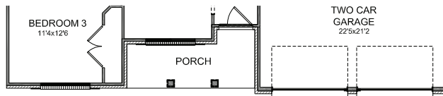
FIRST FLOOR PLAN B
