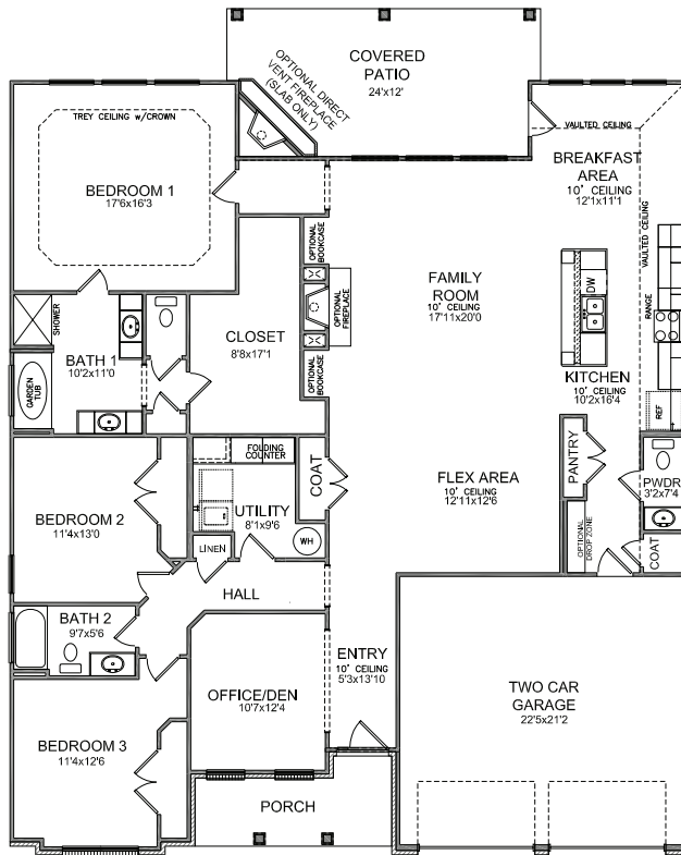
FIRST FLOOR PLAN A
