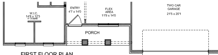
FIRST FLOOR PLAN ELEVATION 'B'
