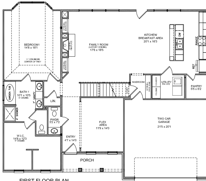
FIRST FLOOR PLAN ELEVATION 'A'
