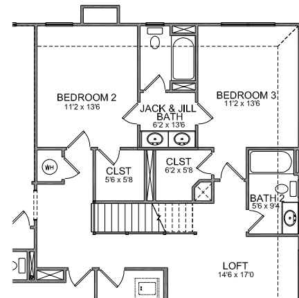
OPTIONAL JACK & JILL BATH WITH BEDROOM 2 AND 3. BATH 2 GOES FROM 60" VANITY TO 42" VANITY
