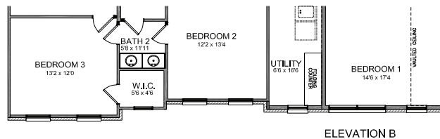
SECOND FLOOR PLAN 9' CEILINGS STANDARD w/10' VAULT IN BEDROOM 1
