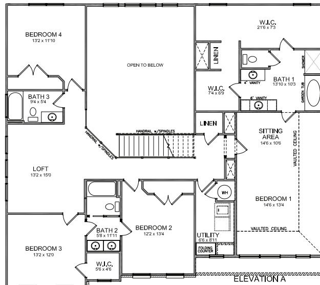
SECOND FLOOR PLAN 9' CEILINGS STANDARD w/10' VAULT IN BEDROOM 1
