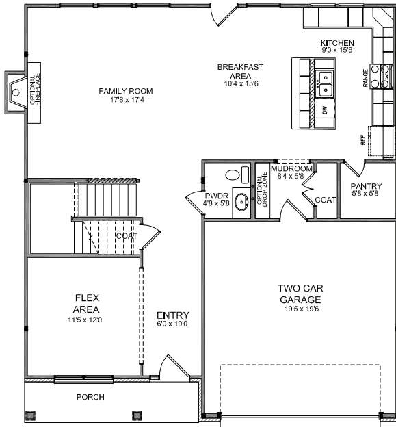
FIRST FLOOR PLAN A
