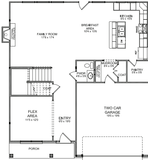
FIRST FLOOR PLAN A
