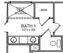
OPTIONAL BATH 1 SHOWN WITH 6'x3'8" FULLY TILED SHOWER, 5010 TRANSOM AND LINEN CLOSET
