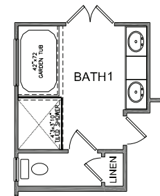
OPTIONAL BATH 1 SHOWN WITH w/42x72 GARDEN TUB & 4'3x3'10 FULLY TILED SHOWER
