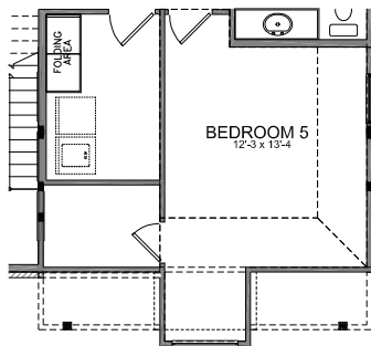
BEDROOM 5 OPTION
