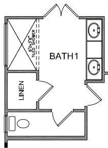
OPTIONAL BATH 1 SHOWN WITH 6'x3'8 FULLY TILED SHOWER AND LINEN CLOSET INCLUDES 5010 TRANSOM OVER SHOWER
