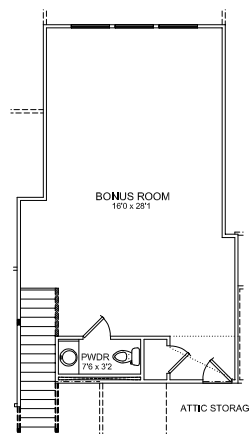
2ND FLOOR OPTIONAL BONUS ROOM LAYOUT WITH POWDER ROOM
