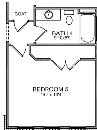
OPTIONAL FIRST FLOOR BEDROOM 5 SHOWN w/OPTION BATH 4 IN LIEU OF STUDY AND POWDER ROOM
