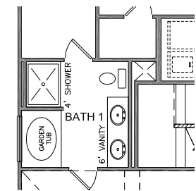
UPGRADED BATH 1 WITH 42X60 GARDEN TUB WITH PICTURE WINDOW ABOVE 4'X3' FIBERGLASS SHOWER
