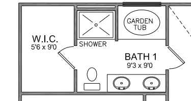
UPGRADED BATH 1 WITH 42X60 GARDEN TUB PICTURE WINDOW ABOVE 4'X3' FIBERGLASS SHOWER
