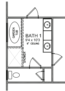
OPTIONAL BATH 1 WITH 36x72 GARDEN TUB, 4'x3'4" FULLY TILED SHOWER
