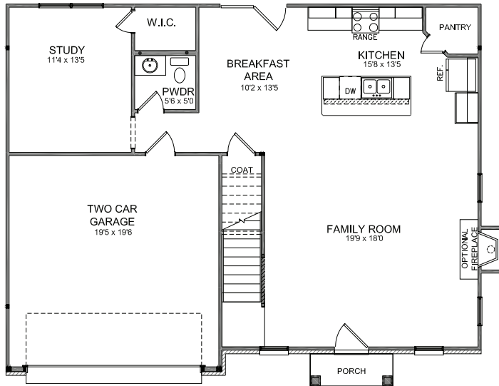
FIRST FLOOR PLAN A & B
