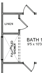
OPTIONAL BATH 1 SHOWN WITH 6'x3'8 FULLY TILED SHOWER, 5010 TRANSOM AND LINEN CLOSET
